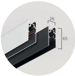
Suspended Track Linear: X-LPQ-840M-L2000-B [BLACK] X-LPQ-840M-L2000-W [WHITE]
